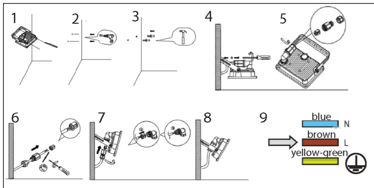
Fig. 2 : Mounting
