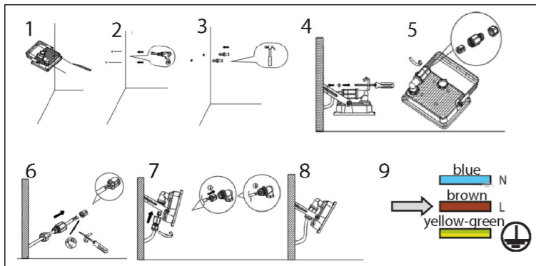
Fig. 2 : Mounting
