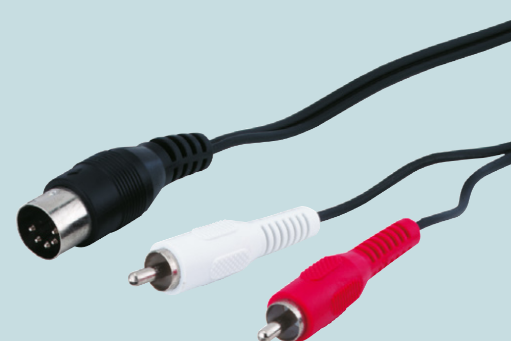
Audio Cable Adapter, DIN Male to Stereo RCA Male DIN male 180° (5-pin) > 2 RCA male (audio left/right)
