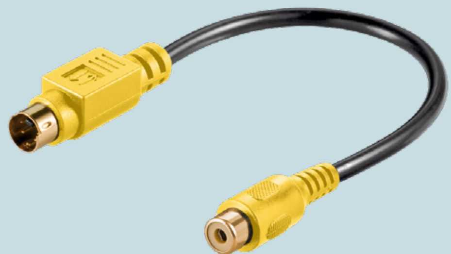
Video Cable Adapter, S-Video to Composite Mini-DIN 4 male (S-Video) > RCA female
